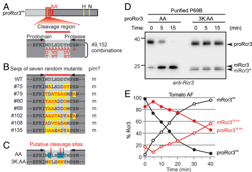
Fig. 6. Asp residues in proRcr3 are required for cleavage by P69B. (A) Random mutagenesis of the cleavage region in proRcr3. ProRcr3 3K:AA was synthesized with specific degenerate codons in the region encoding the putative cleavage site in proRcr3. All possible amino acid substitutions are shown in red. There are 49,152 possible combinations of these substitutions and original residues. (B) All tested random mutants accumulate as mRcr3 on agroinfiltration. A total of 315 random mutants were transiently expressed in N. benthamiana by agroinfiltration, and total extract was isolated and analyzed by Western blot using the anti-Rcr3 antibody. Shown are sequences of seven random clones, indicating that the mutagenesis was successful. (C) Mutant proRcr3 3K:AA carries three Asp-into-Lys substitutions in the putative cleavage region of proRcr3 3K:AA . (D) Purified proRcr3 3K:AA is no longer cleaved by purified P69B in vitro. (E) Processing of purified proRcr3 3K:AA is slower when incubated with AF of tomato.
