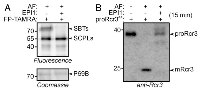
Fig. 4. SBT inhibition by P. infestans effector EPI1 blocks Rcr3 AA maturation. (A) EPI1 blocks SBT labeling in tomato AF. AF from Cf2/ rcr3 tomato plants was incubated with and without 17 \mu M purified EPI1 for 1 h and then labeled with 0.2 \mu M FP for 1 h. Proteins were separated by SDS-PAGE and analyzed by fluorescence scanning and Coomassie staining. (B) EPI1 blocks Rcr3 maturation. AF from Cf2/ rcr3 tomato plants was incubated with 17 \mu M purified EPI1 for 1 h and then incubated with purified proRcr3 AA . Samples were taken after 15 min and analyzed by Western blot using the anti-Rcr3 antibody.
